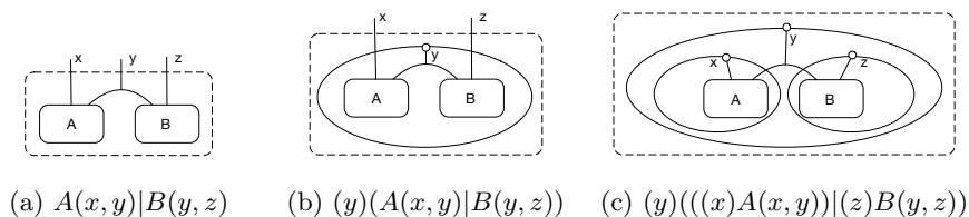
Fig. 3: Some examples of bigraphs
